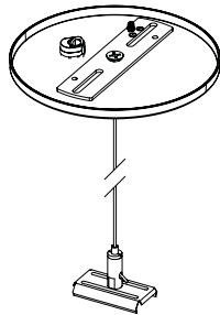
PW-PC-01 Pendant wire, Power side with clips, canopy 70 inches
